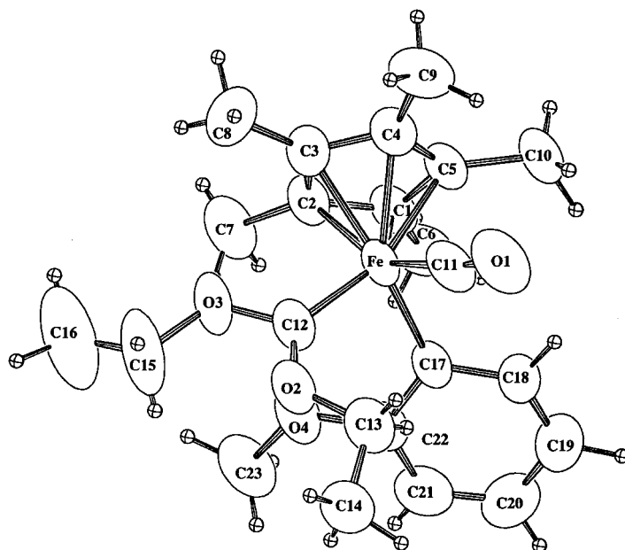
Figure 2. Crystal structure of 8 . Selected bond lengths [Å] and angles [°]: Fe–C17 1.990(6), Fe–C12 1.881(5), O2–C12 1.305(7), O3–C12 1.335(7), O4–C23 1.423(7); Fe–C11–O1 173.2(6), O2–C12–O3 108.8(4), Fe–C12–O2 133.4(4), Fe–C12–O3 117.8(4).
