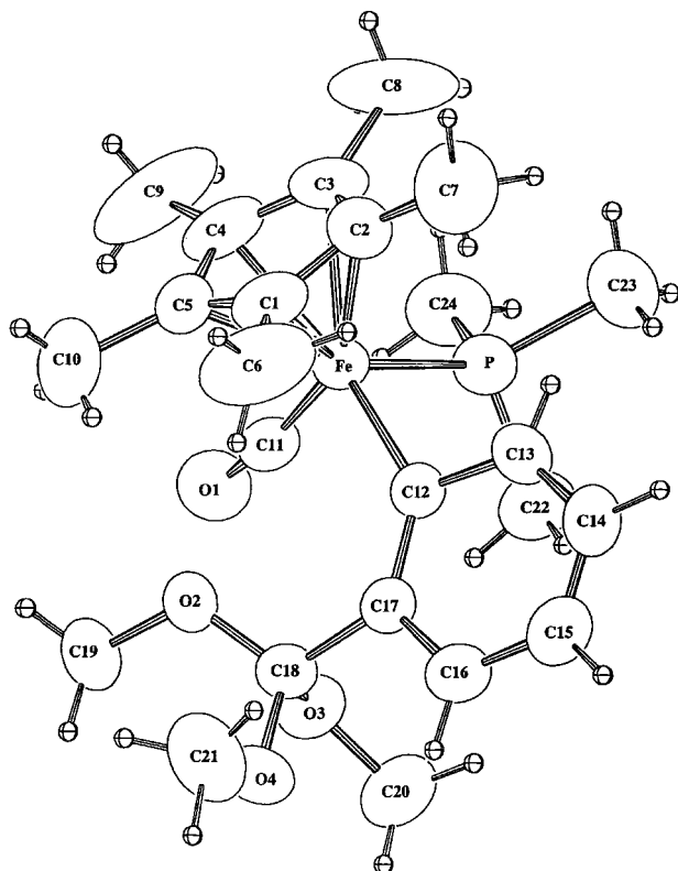
Figure 1. Crystal structure of 4 . Selected bond lengths [Å] and angles [°]: C17–C18 1.519(6), O2–C18 1.382(4), O3–C18 1.411(4), O4–C18 1.413(5), Fe–C12 2.033(3), Fe–P 2.187(1), Fe–C11 1.699(4), O2–C19 1.426(6), O3–C20 1.420(4), O4–C21 1.421(5); Fe–C11–O1 171.0(3), C11–Fe–C12 99.6, P–Fe–C11 85.9(1), P–Fe–C12 89.2(1), Fe–C12–C17 133.3(3), Fe–C12–C13 112.6(2).
